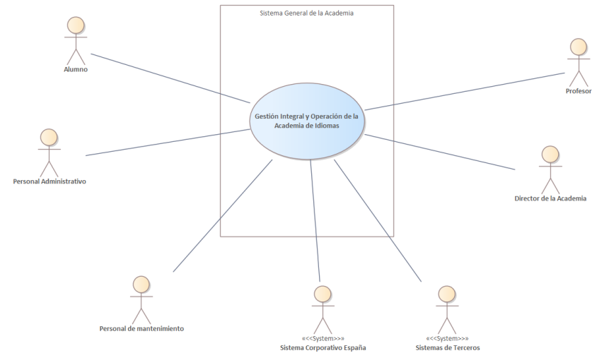
Figure 1: 0UseCaseModel
