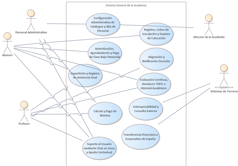
Figure 2: 1UseCaseModel
